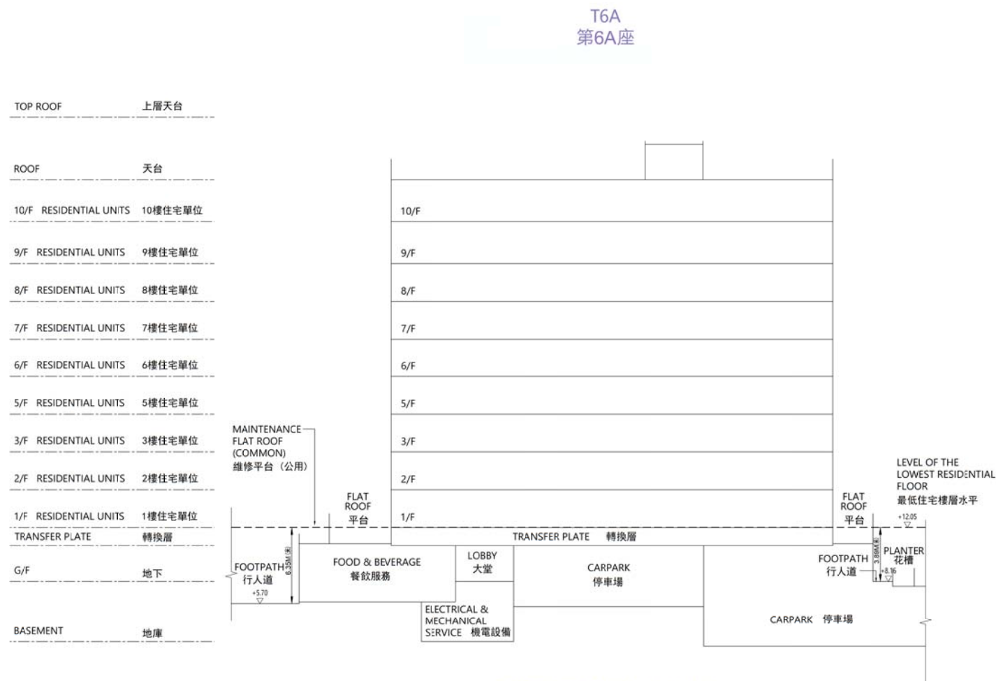
CROSS-SECTION PLAN A2 橫截面圖 A2
