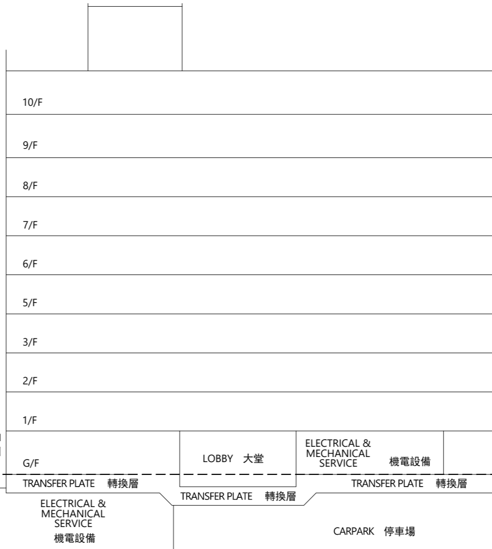
CROSS-SECTION PLAN A2 橫截面圖 A2
