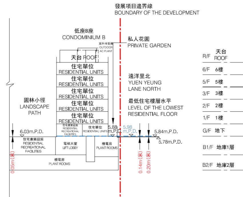
橫截面圖 E-E' Section E-E'
